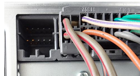
Fig. 2 Radio connector
