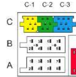
Fig. 1 Radio Connectors
